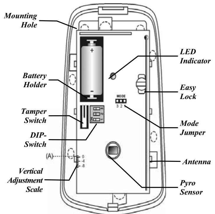
Figure B.1: PIR Sensor with Cover Removed
