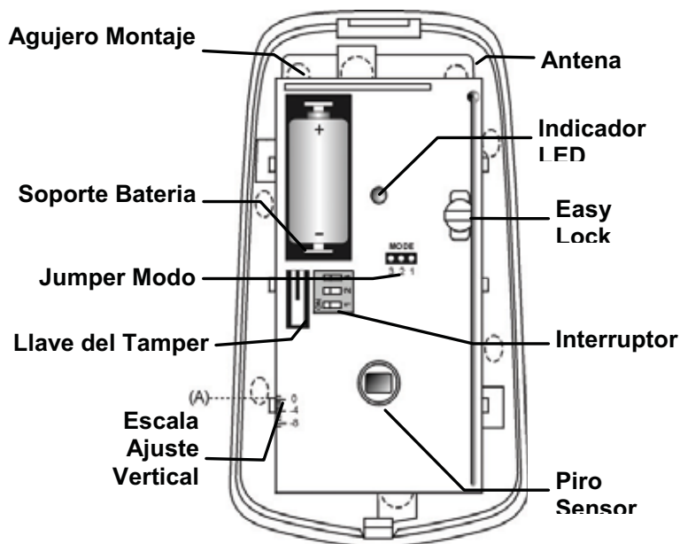
Figura B.1: EL-2600/EL-2600PI (sin tapa)
